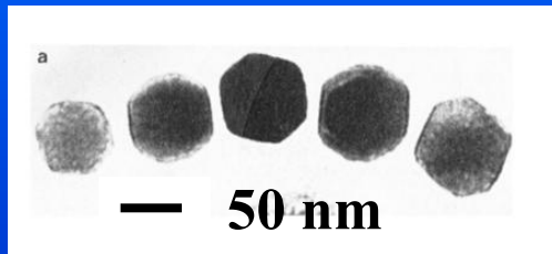
Hexagonal
